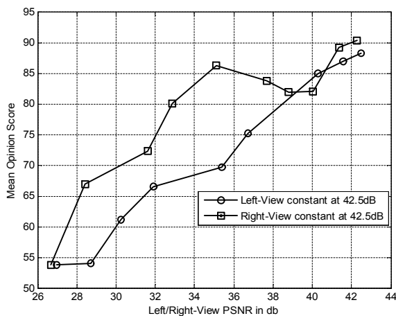
Figure 2. Mean Opinion Scores for Asymmetric View Coding
